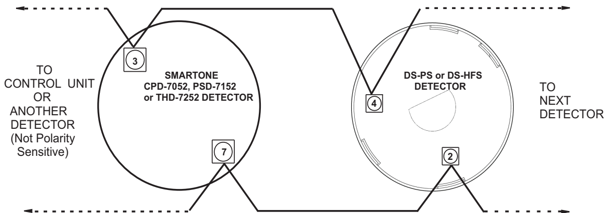
Figure 1: Combining Legacy Detectors with DS Series Detectors (Class B Wiring Style Shown)
